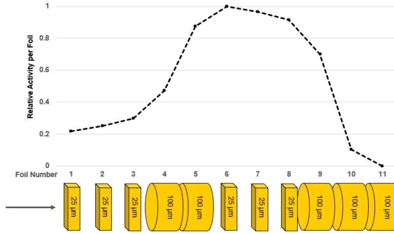
Figure 9: Normalized ^{65}\text{Zn} activity per foil based on MCNP6 foil activation simulation. The line is included to guide the eye.
